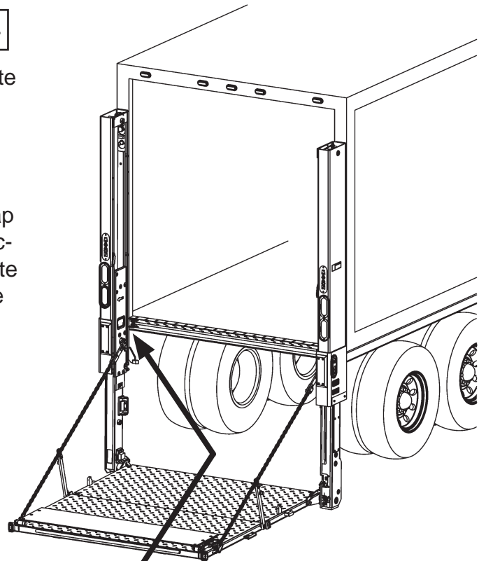
LOWERING LIFTGATE FIG. 73-1
