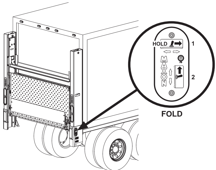
PRESSURIZING CLOSING CYLINDER FIG. 61-2
