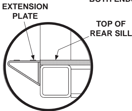
FLUSH EXTENSION PLATE FIG. 20-3
