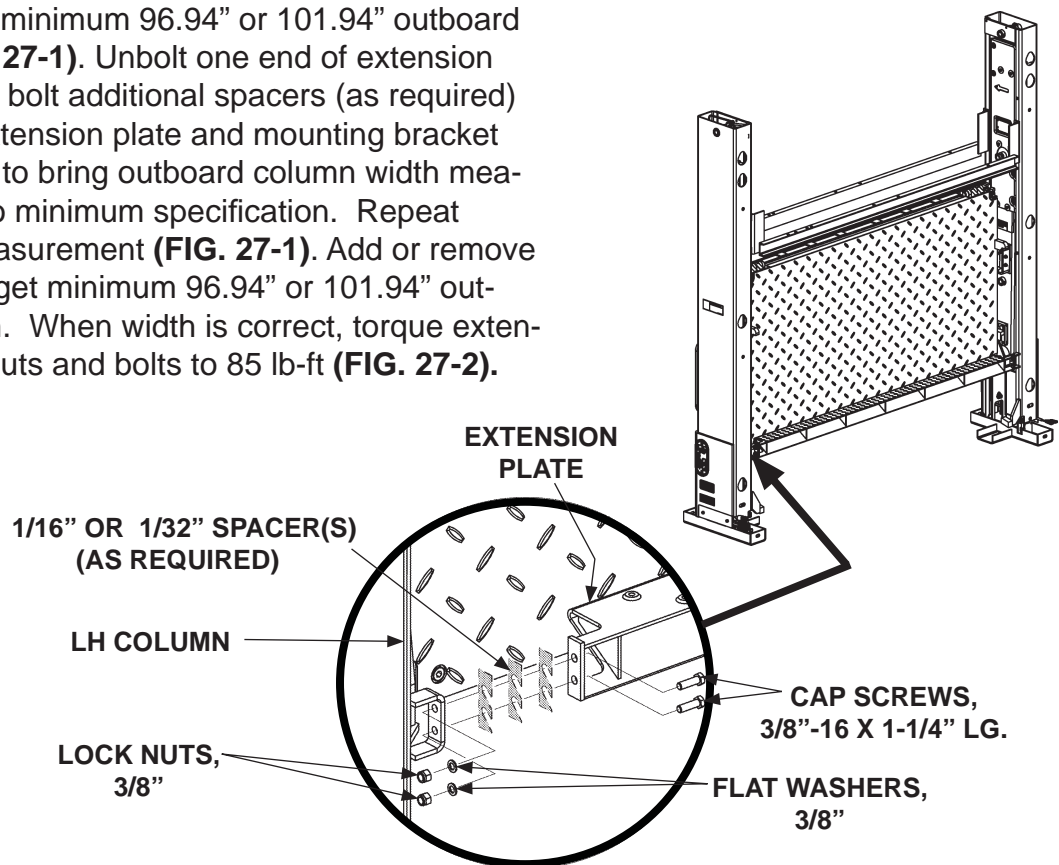
ADDING OR REMOVING SPACERS FIG. 27-2
