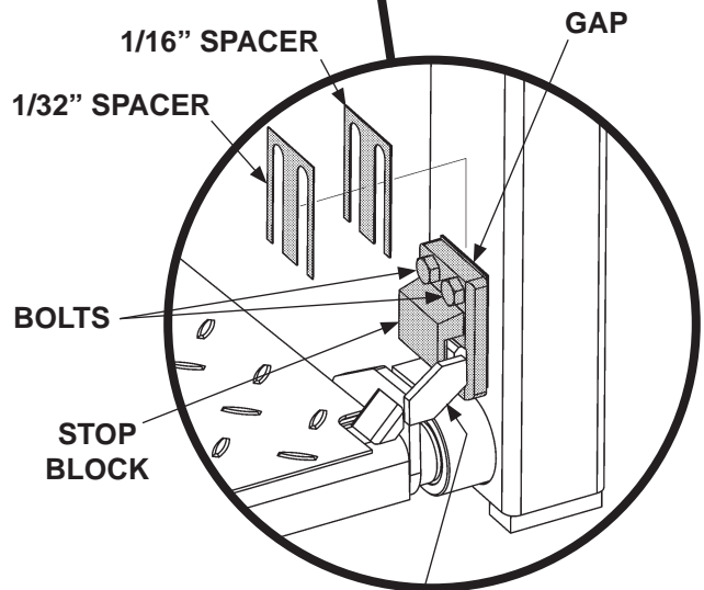
MOUNTING BRACKET
