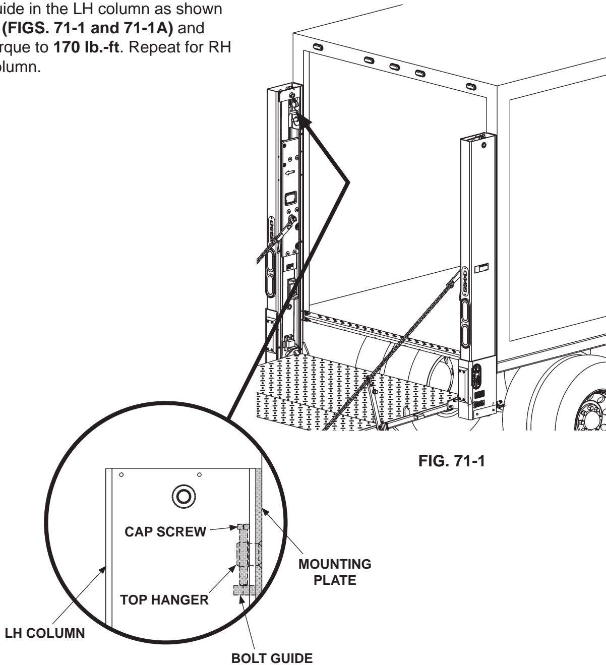
TIGHTENING CAP SCREW FIG. 71-1A
