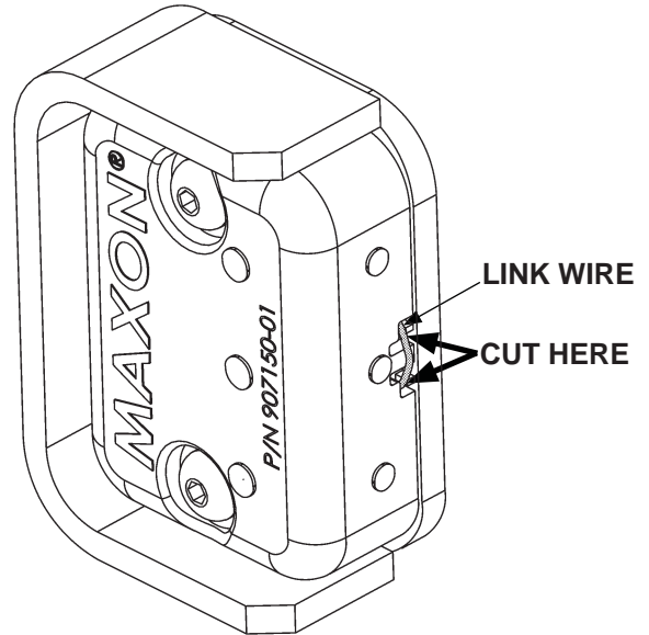
ACTIVATING PLATFORM LIGHTS FIG. 83-1
