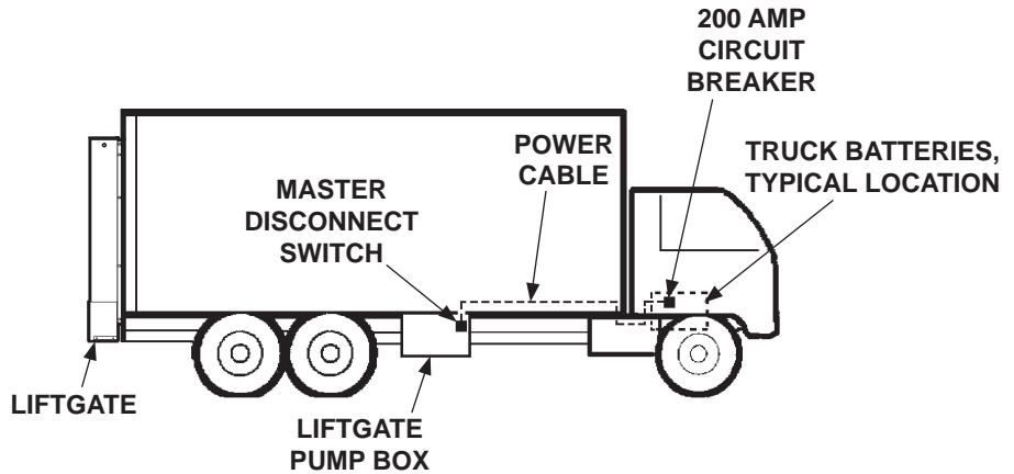
RECOMMENDED LIFTGATE INSTALLATION ON TRUCK
