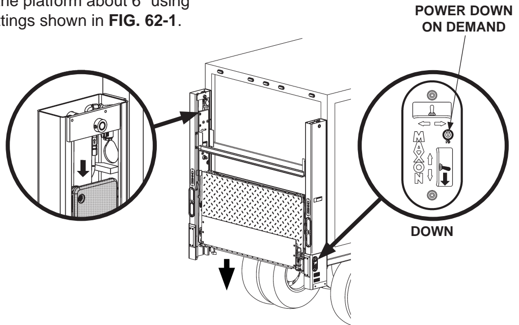
LOWERING PLATFORM FIG. 62-1
