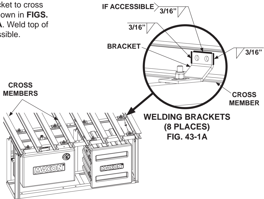
BOLTING PUMP & BATTERY BOX FRAME FIG. 43-1
