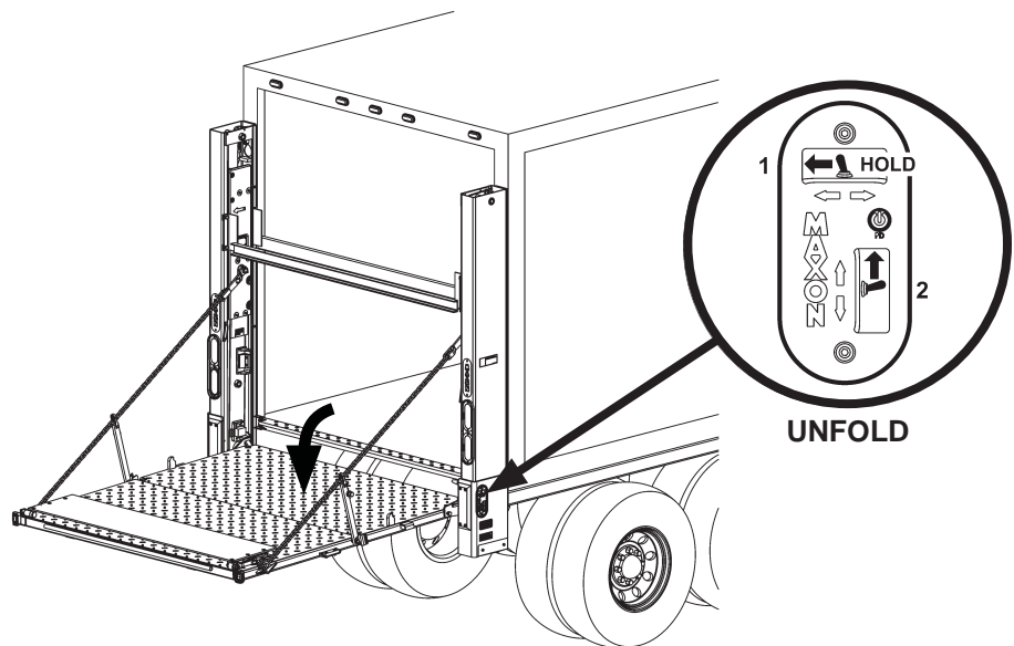
UNFOLDING PLATFORM FIG. 62-2
