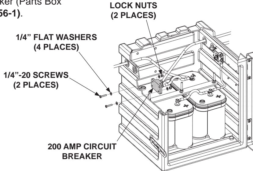
BATTERY BOX FIG. 56-1
