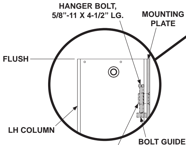
INSERTING CAP SCREW INTO LH TOP HANGER FIG. 36-1B
