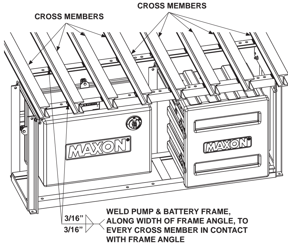
ALIGNING PUMP & BATTERY BOX FRAME TO WELD ON CROSS MEMBERS FIG. 44-1
