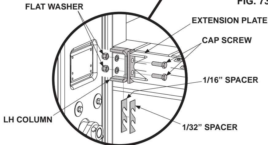
REINSTALLING HARDWARE FIG. 73-1A
