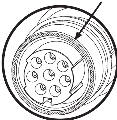
DIELECTRIC GREASE ON RECEPTACLE FIG. 52-4
