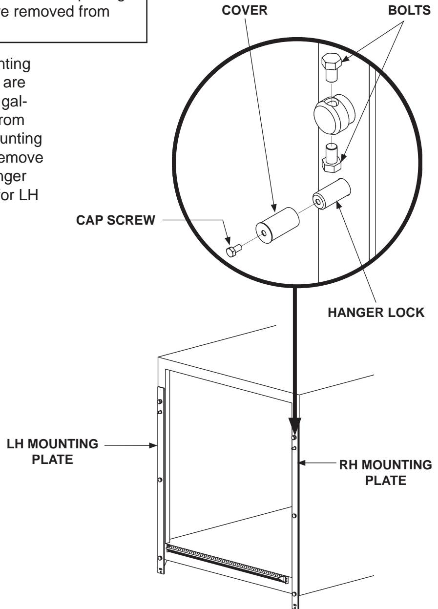
LIFTGATE MOUNTING PLATES FIG. 33-1
