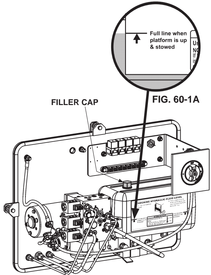
PUMP BOX SHOWN WITH SINGLE PUMP FIG. 60-1
