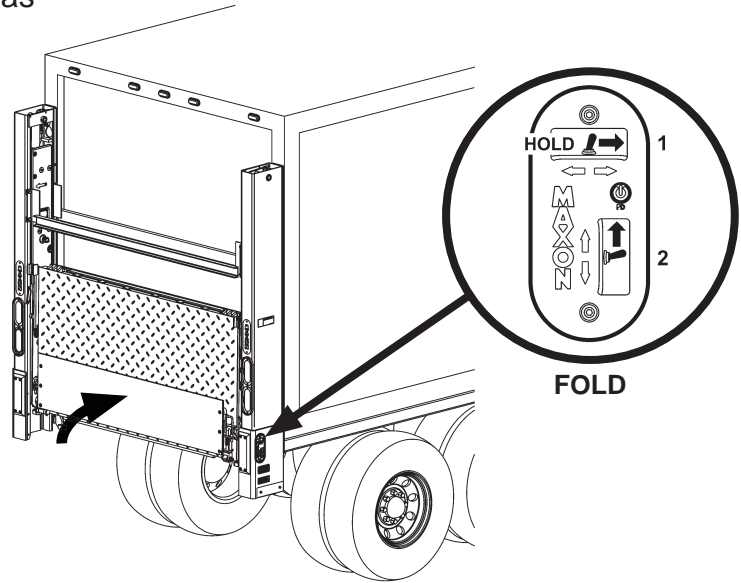
FOLDING PLATFORM FIG. 63-1
