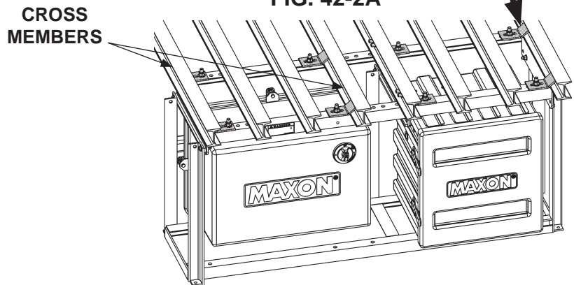
BOLTING PUMP & BATTERY BOX FRAME FIG. 42-2
