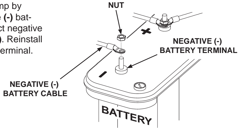
DISCONNECTING POWER FIG. 75-1
