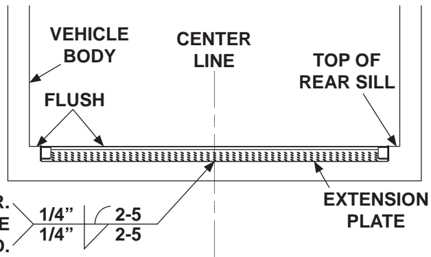
CENTERING EXTENSION PLATE ON 96" WIDE VEHICLE BODY FIG. 20-1
