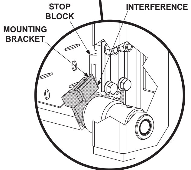
REAR VIEW OF LH RUNNER FIG. 67-1A
