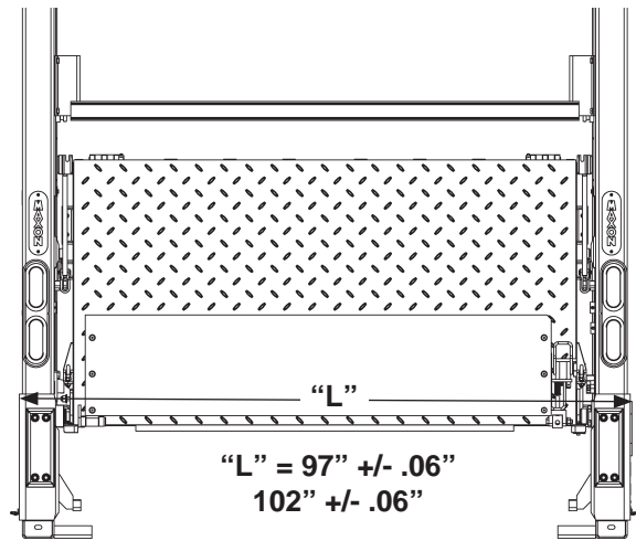
MEASURING OUTBOARD WIDTH AT COLUMN REINFORCEMENTS FIG. 27-1
