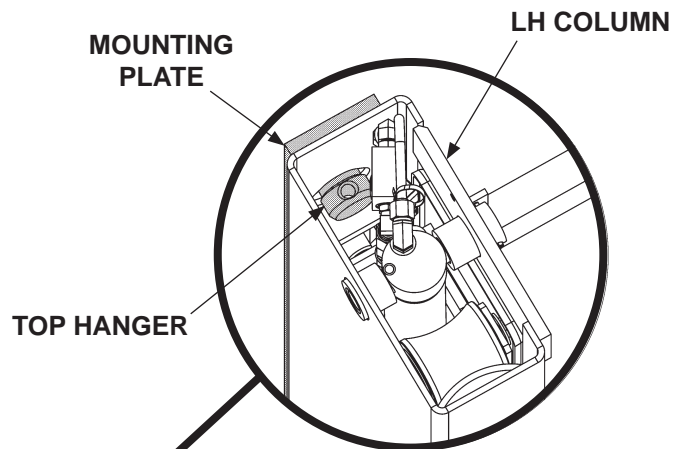
LOCATING LH TOP HANGER FIG. 36-1A
