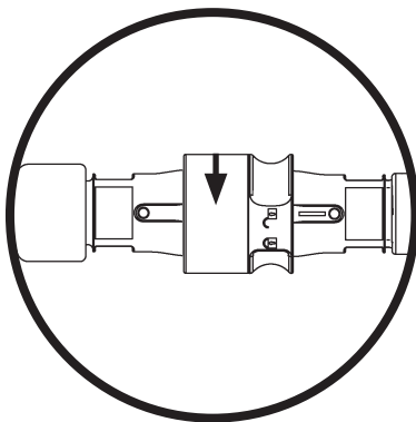
TWIST COUPLING RING TO UNLOCK FIG. 52-1
