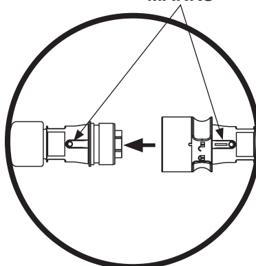
ALIGN & CONNECT FIG. 52-5
