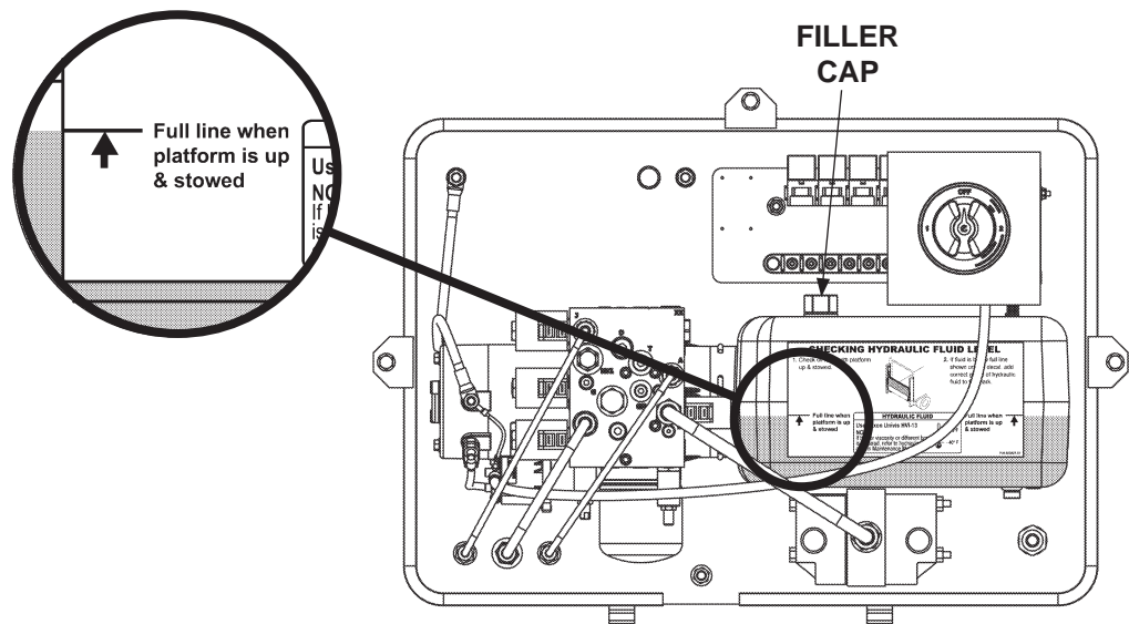
CHECKING HYDRAULIC FLUID LEVEL FIG. 66-1
