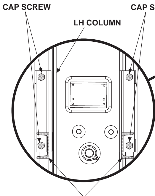
SUPPORT CHANNEL LOOSENING LH SUPPORT CHANNELS FIG. 35-1A
