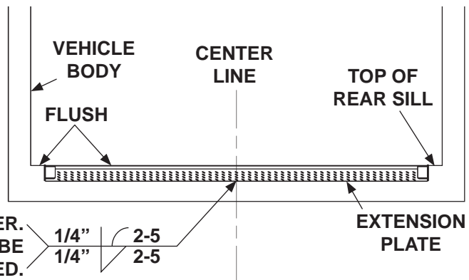
CENTERING EXTENSION PLATE ON 102" WIDE VEHICLE BODY FIG. 20-2
