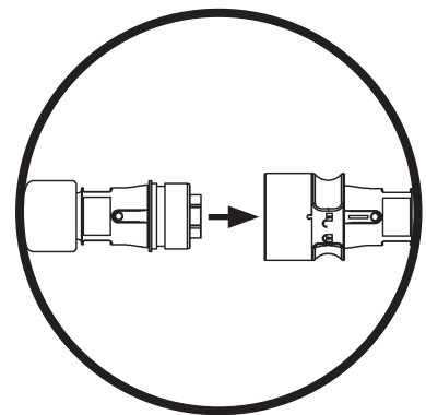
PULL CONNECTORS TO DISCONNECT FIG. 52-3
