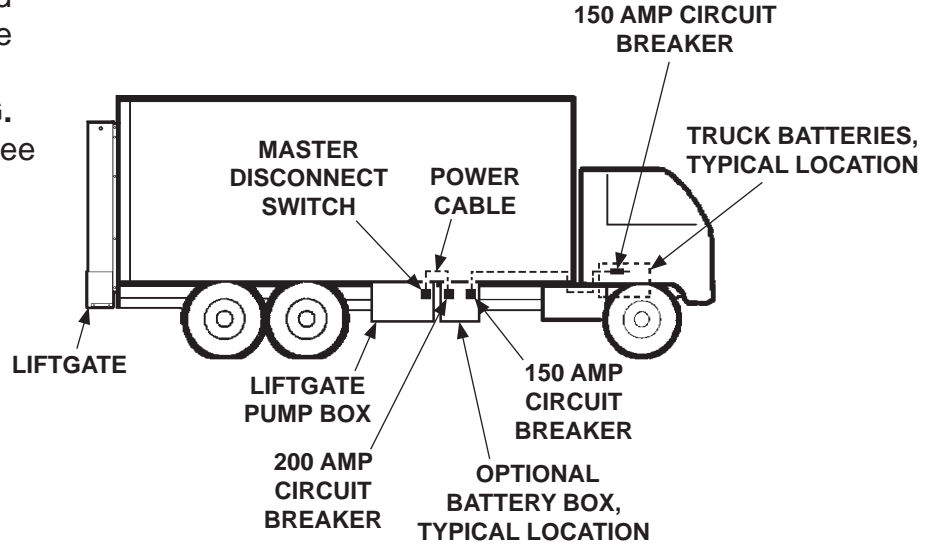
RECOMMENDED LIFTGATE & BATTERY BOX INSTALLATION ON TRUCK
