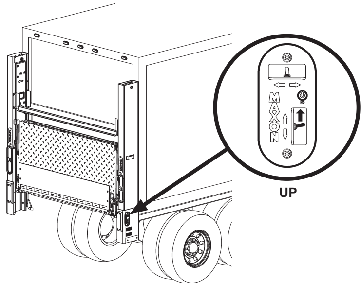
RAISING PLATFORM FIG. 65-2
