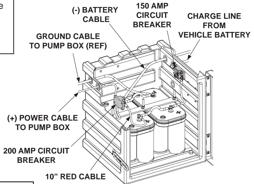
BATTERY BOX FIG. 59-1
