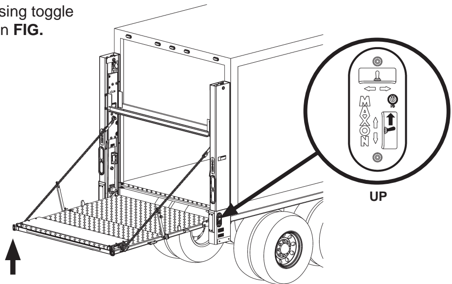
RAISING PLATFORM FIG. 64-2
