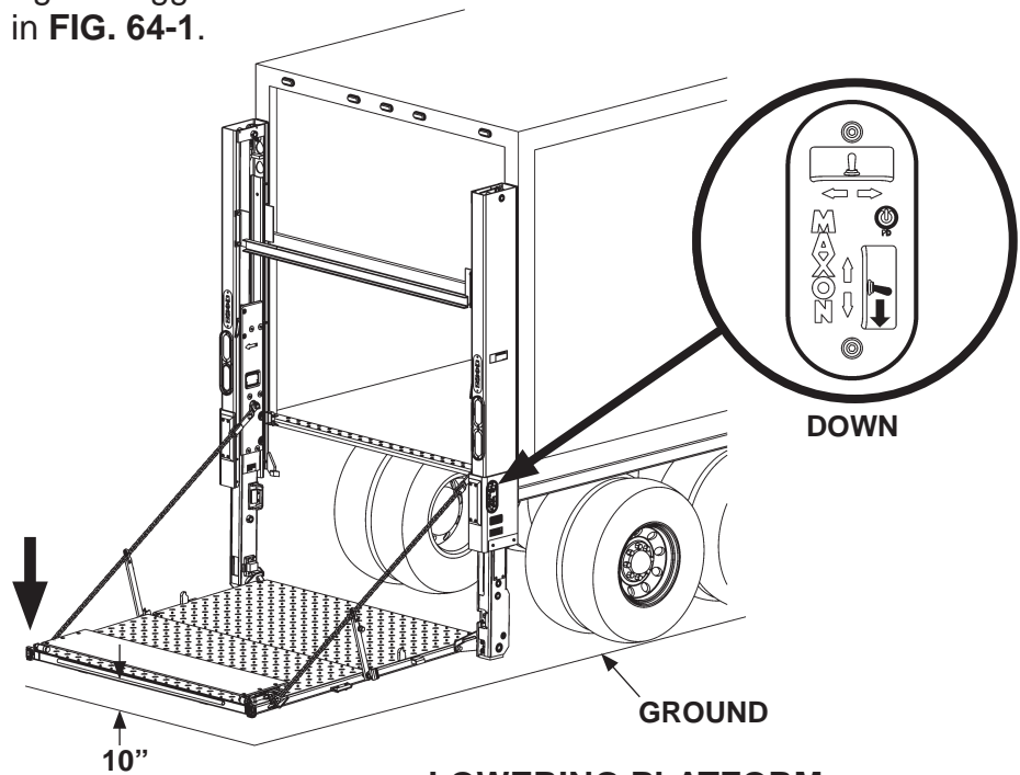
LOWERING PLATFORM FIG. 64-1
