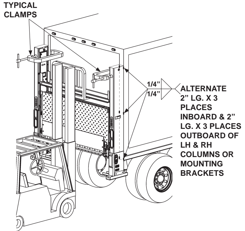
WELDING LIFTGATE TO VEHICLE FIG. 31-1
