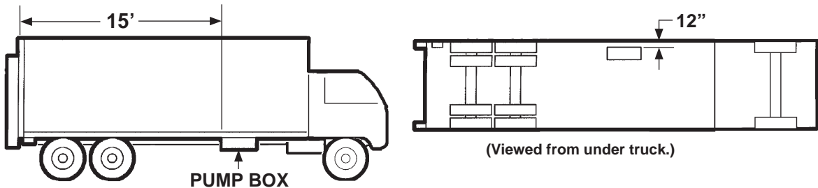
TYPICAL 15 FT. INSTALLATION FIG. 38-3
