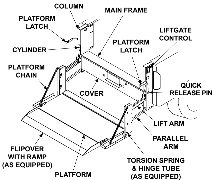
C2 PICKUP LIFTGATE SHOWN FIG. 8-1
