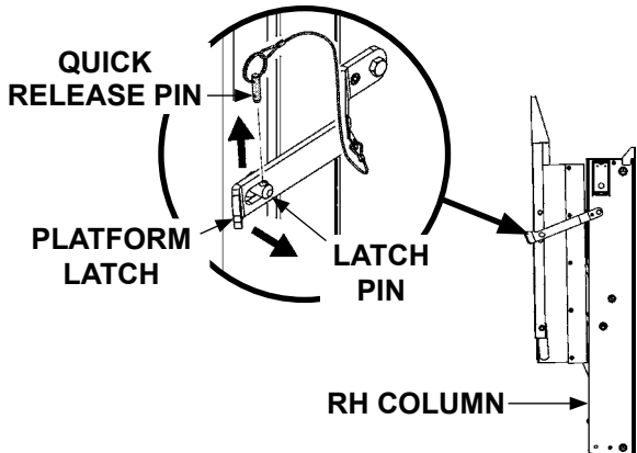
UNLATCHING PLATFORM FROM RH COLUMN FIG. 14-2
