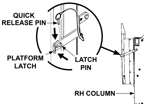
LATCHING PLATFORM TO RH COLUMN FIG. 20-1
