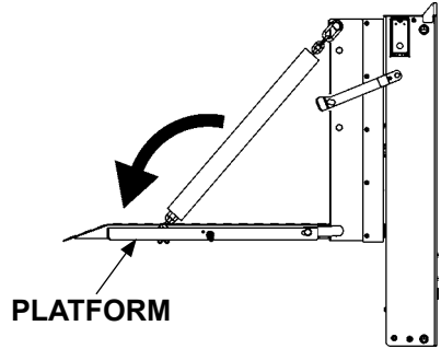
UNFOLDING PLATFORM (RH SIDE VIEW) FIG. 15-1
