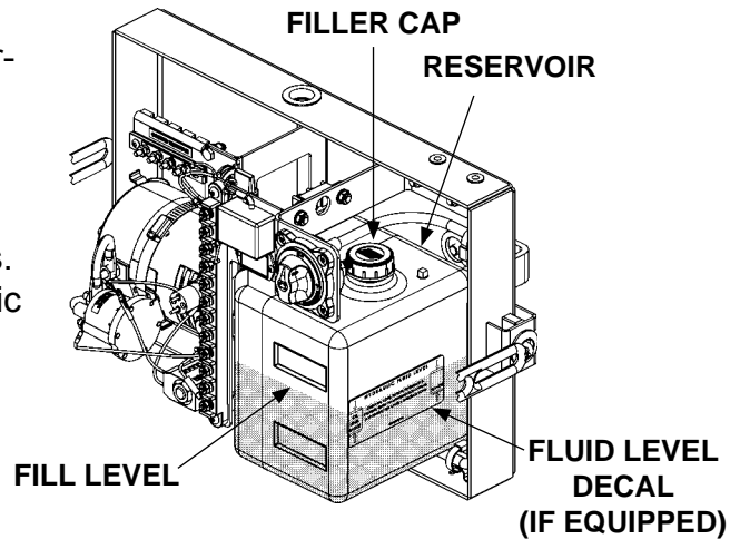
FILL PUMP RESERVOIR FIG. 17-1
