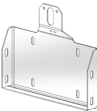
LICENSE PLATE BRACKET P/N 287014-01 QTY. 1
