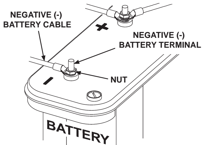
RECONNECTING POWER FIG. 4-1
