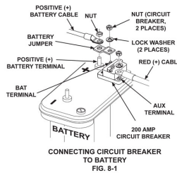
BATTERY JUMPER (CIRCUIT BREAKER MOUNT) P/N 295967-01 QTY. 1
