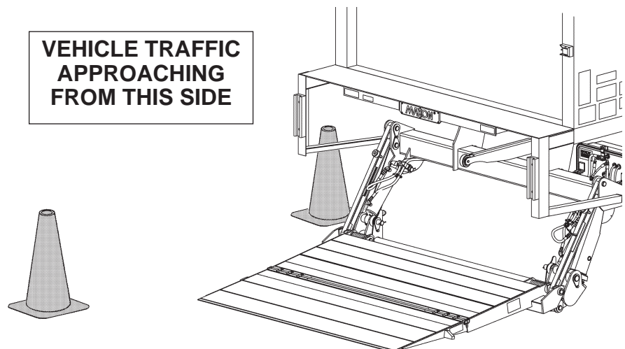
TRAFFIC CONES POSITIONED BY PLATFORM LOADING AREA (GPT LIFTGATE SHOWN)
