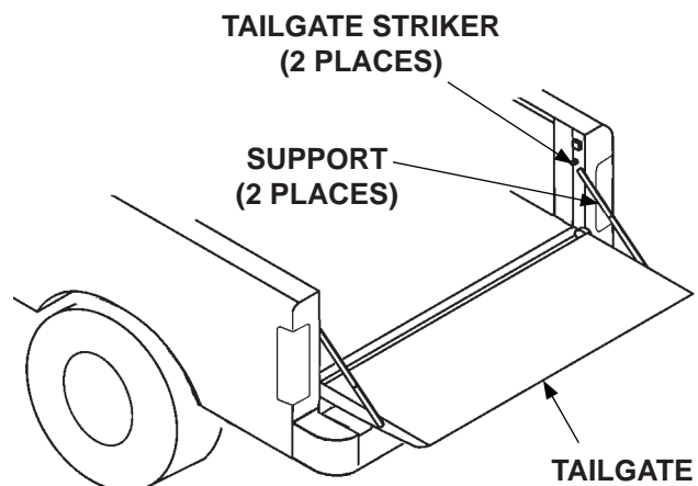
REMOVING TAILGATE & SUPPORTS FIG. 10-1
