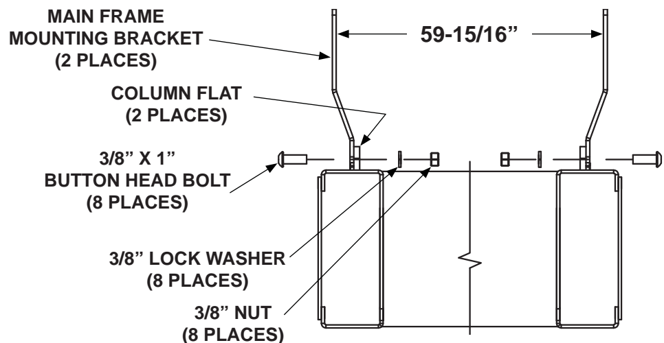
BOLTING MAIN FRAME MOUNTING BRACKETS TO OUTSIDE OF COLUMNS ON C2 LIFTGATE (TOP VIEW) FIG. 9-2
