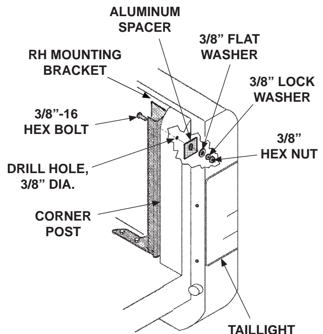
BOLTING RH MOUNTING BRACKET TO PICKUP BED (LIFTGATE NOT SHOWN) FIG. 14-1
