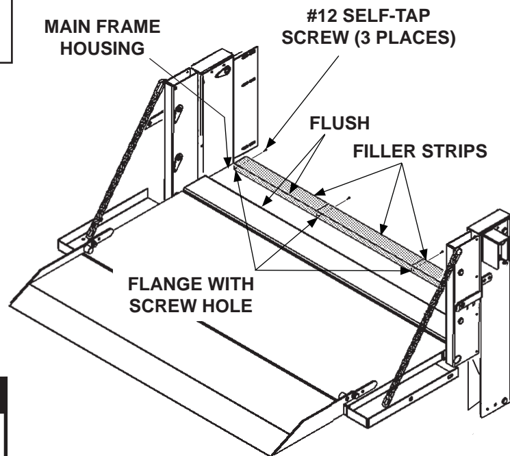
POSITIONING FILLER STRIPS FIG. 11-1
