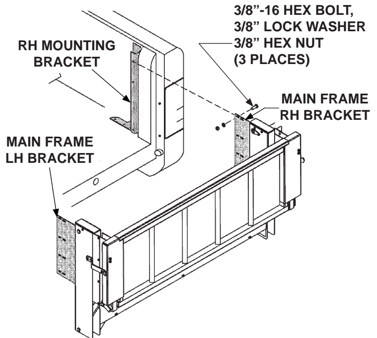
BOLTING LIFTGATE TO RH MOUNTING BRACKET FIG. 12-2
