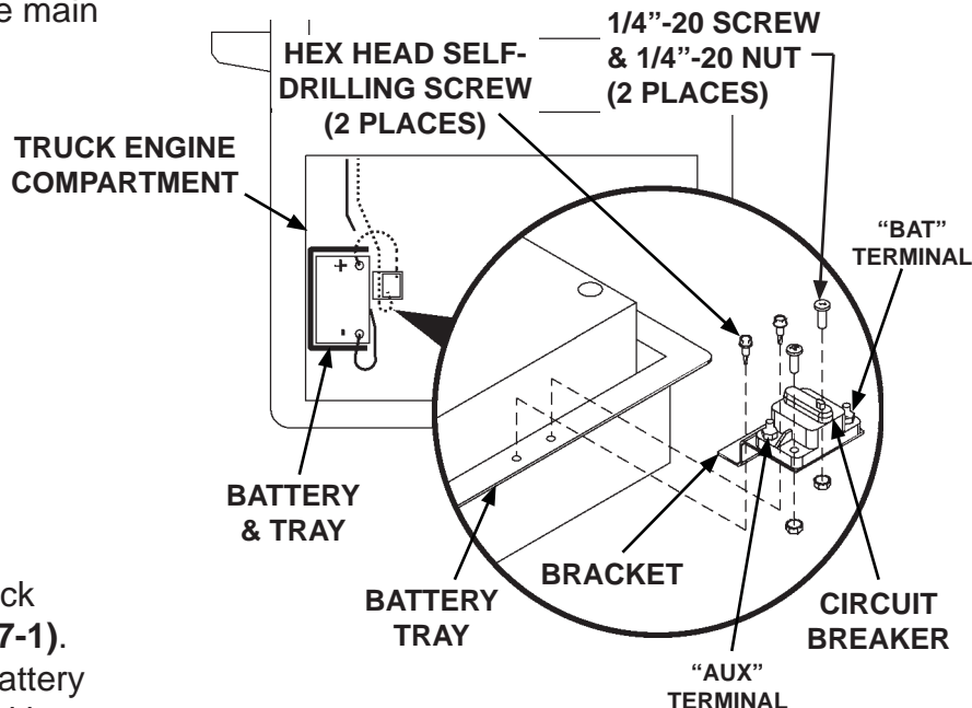
BOLTING CIRCUIT BREAKER & BRACKET TO TRUCK BATTERY TRAY (TOP VIEW) FIG. 17-2
