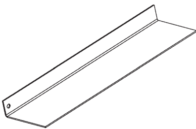
19-1/2" LG FILLER PLATE, GALVANIZED P/N 297888-02 QTY. 3
