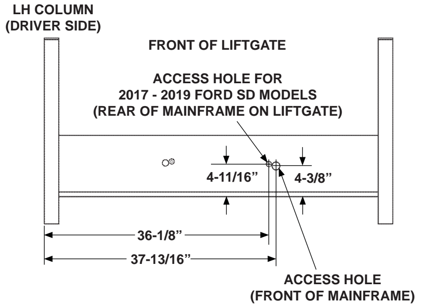
REMOVING PLASTIC PLUGS FOR SPARE TIRE ACCESS, FORD SUPER DUTY F-250, F-350 & F-450 MODELS (2017 - 2019) FIG. 16-1
