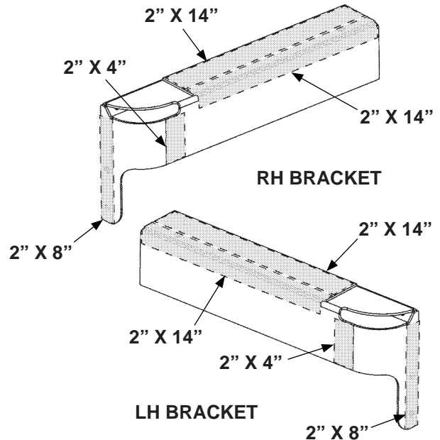
TAPING MOUNTING BRACKETS FIG. 12-1
