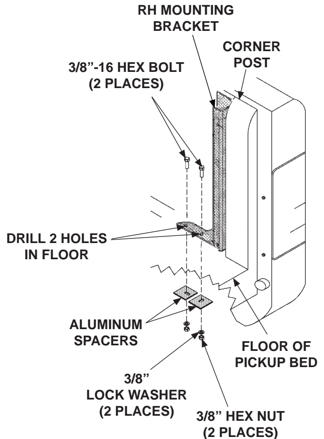
BOLTING RH MOUNTING BRACKET TO PICKUP BED (LIFTGATE NOT SHOWN) FIG. 13-1
