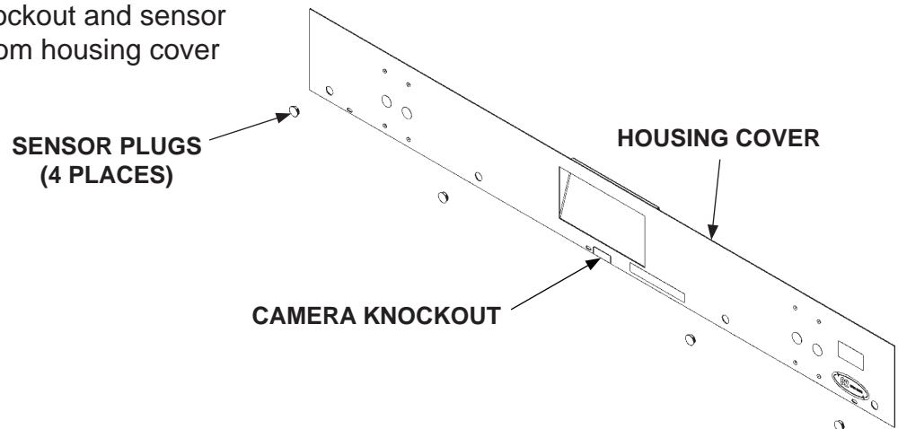
REMOVING HOUSING COVER SENSOR PLUGS AND CAMERA KNOCKOUT FIG. 21-1
