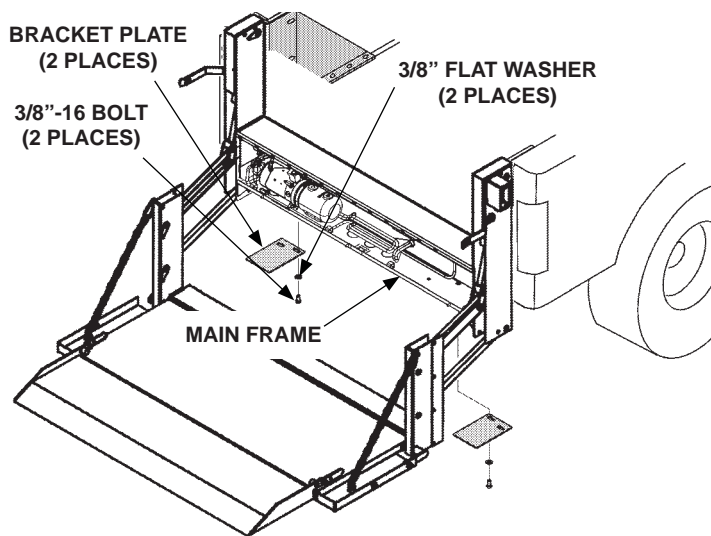
REMOVING BRACKET PLATES FROM MAIN FRAME HOUSING (C2 SHOWN) FIG. 22-1
