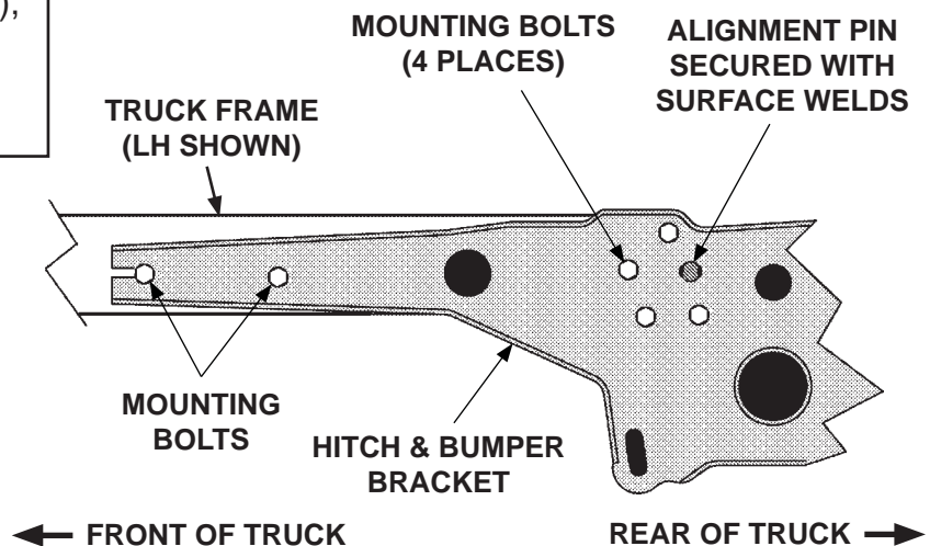
HITCH & REAR BUMPER BRACKET VIEWED FROM OUTER LH SIDE OF TRUCK FRAME FIG. 9-2
