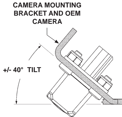
ADJUSTING CAMERA ANGLE FIG. 20-1
