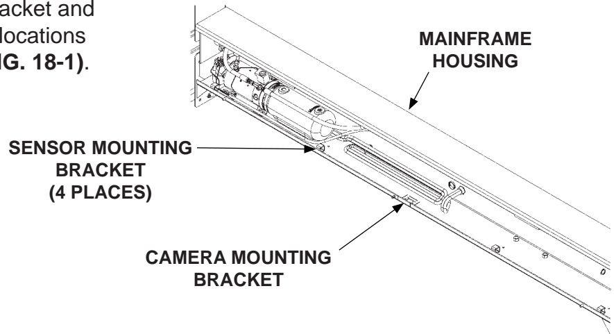
CAMERA AND SENSOR BRACKET LOCATION FIG. 18-1
