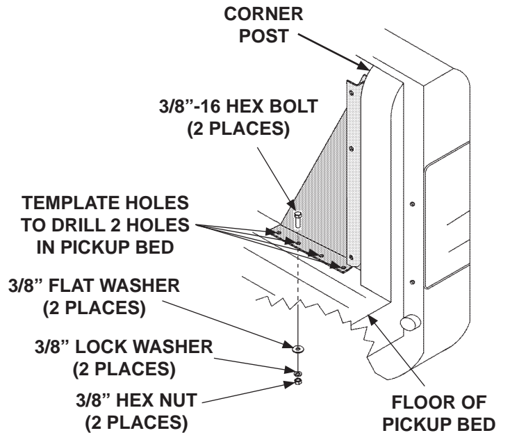
BOLTING RH MOUNTING BRACKET TO PICKUP BED (LIFTGATE NOT SHOWN) FIG. 13-1
