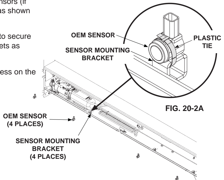
INSTALLING SENSORS (IF EQUIPPED) FIG. 20-2
