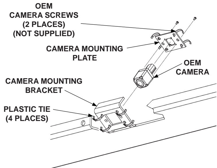
ATTACHING CAMERA TO MOUNTING PLATE AND MOUNTING BRACKET FIG. 19-2
