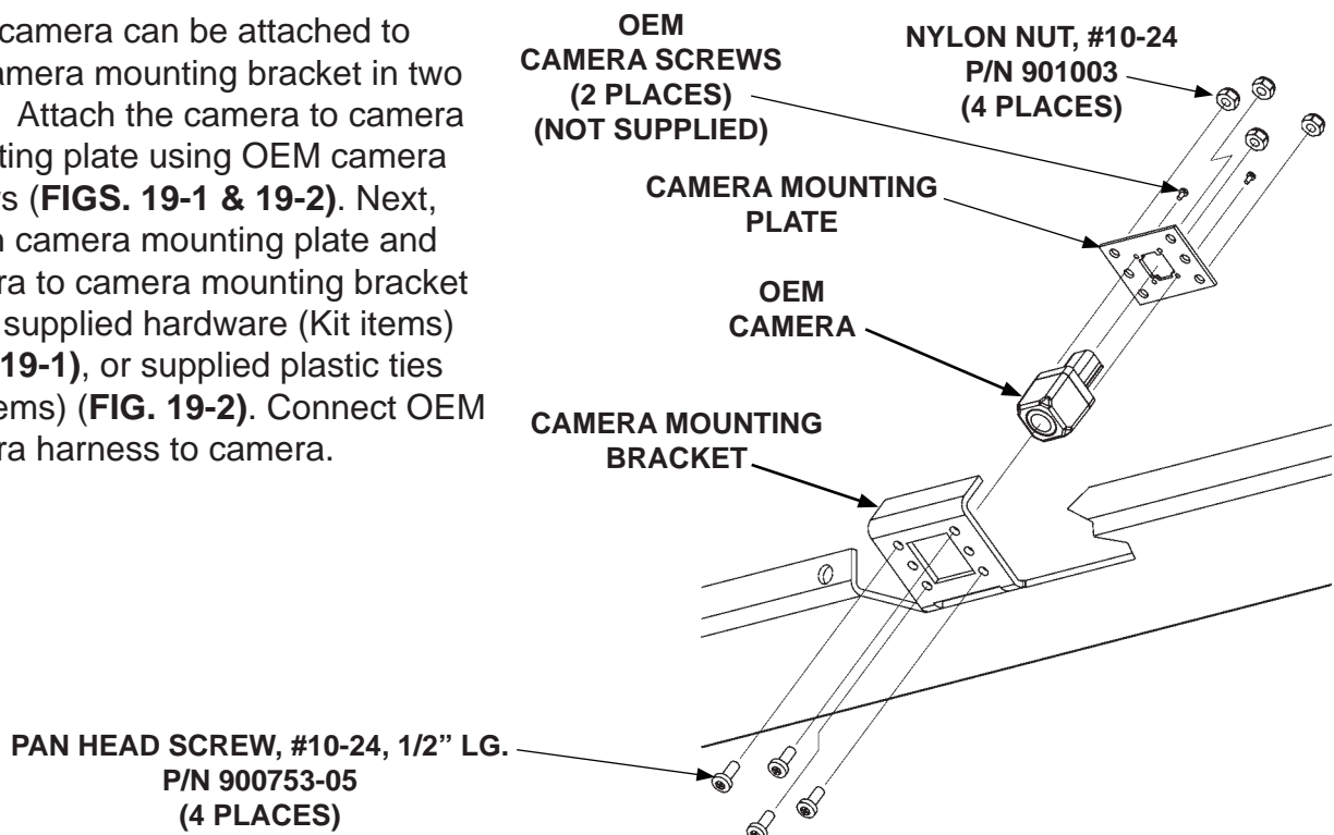
ATTACHING CAMERA TO MOUNTING PLATE AND MOUNTING BRACKET FIG. 19-1
