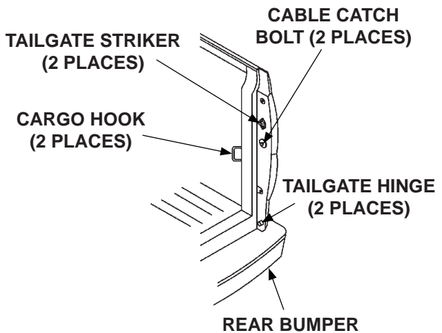
REMOVING TAILGATE & SUPPORTS FIG. 9-1
