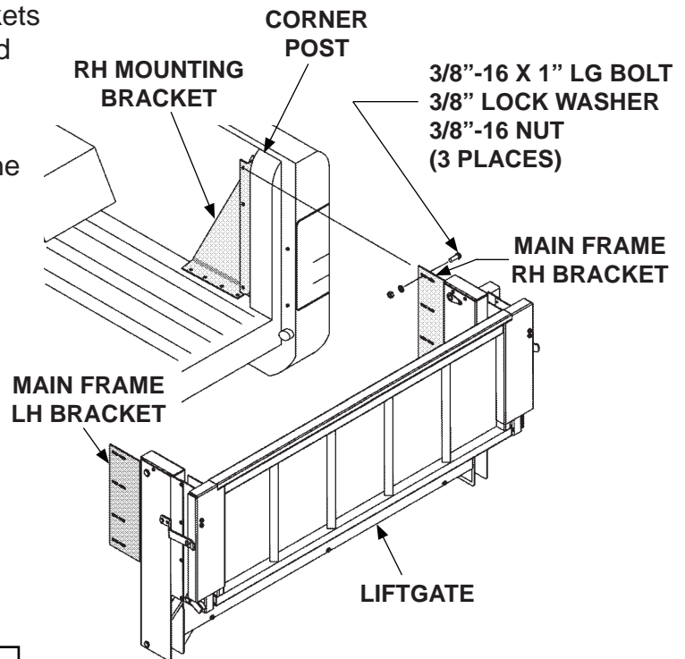
BOLTING LIFTGATE TO RH MOUNTING BRACKET FIG. 12-1
