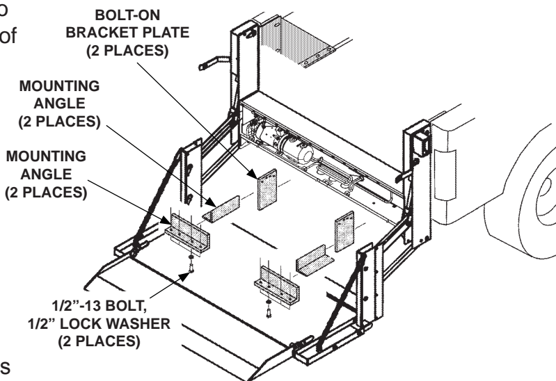
FABRICATING LOWER BRACKETS TO SUPPORT LIFTGATE (C2 SHOWN) FIG. 22-2
