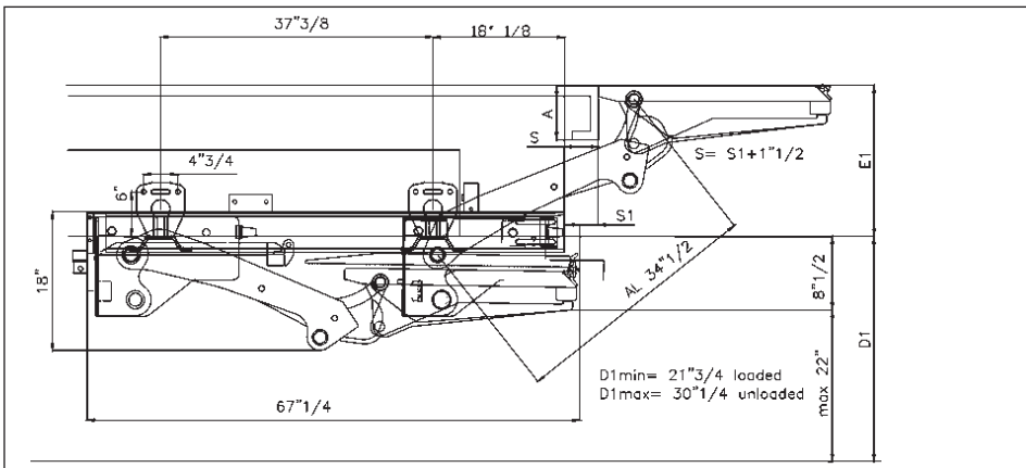
GPST-44 Lift Dimensions and Mounting Requirements
