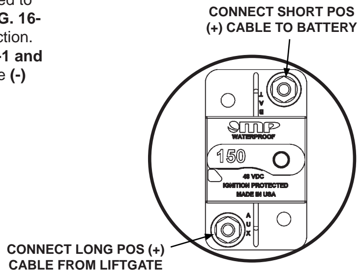
POWER CABLE CONNECTIONS TO 150A CIRCUIT BREAKER
