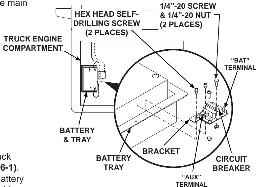
BOLTING CIRCUIT BREAKER & BRACKET TO TRUCK BATTERY TRAY (TOP VIEW) FIG. 16-2
