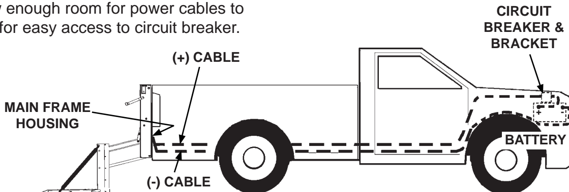
RUNNING POWER CABLES FROM LIFTGATE TO BATTERY FIG. 16-1
