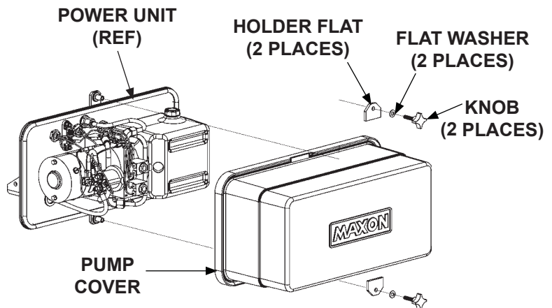
BOLTING / UNBOLTING PUMP COVER FIG. 6-2
